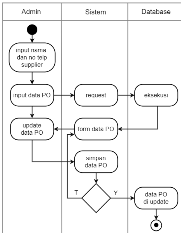
Gambar 5. Activity diagram membuat purchase order (PO)
