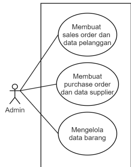
Gambar 3. Usecase diagram
