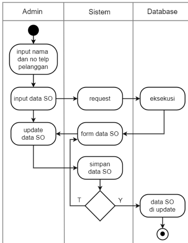
Gambar 4. Activity diagram membuat sales order (SO)
