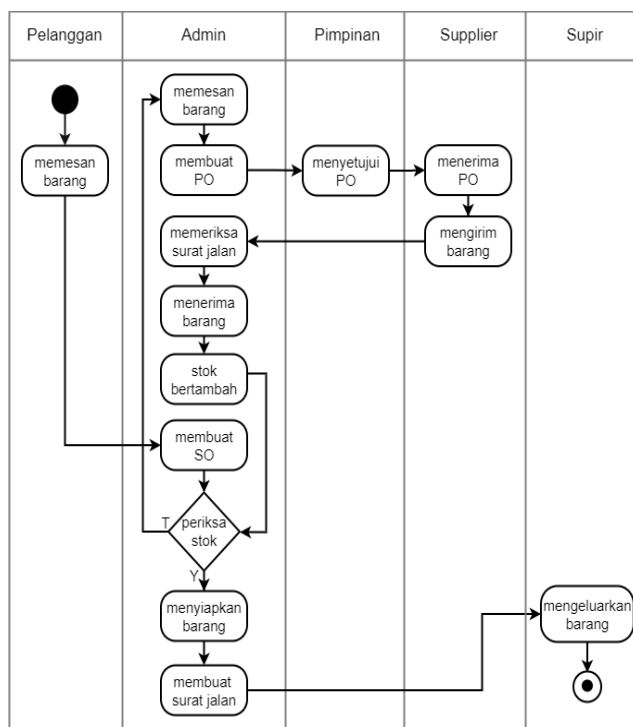
Gambar 2. Activity diagram proses bisnis sistem berjalan
