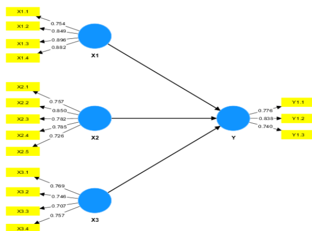
Gambar 1. Hasil Uji Outer Model
