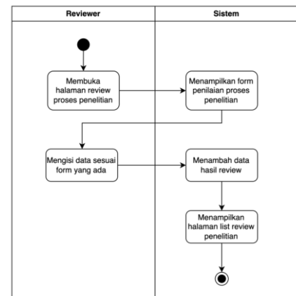
Gambar 5. Activity diagram review proses penelitian
