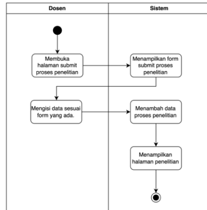
Gambar 4. Activity diagram submit proses penelitian
