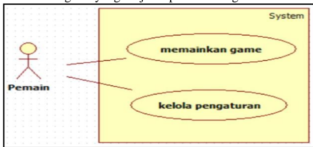
Gambar 2. Usecase Diagram Go Vegetarian
