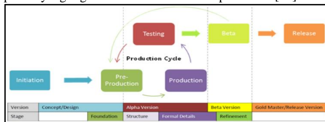
Gambar 1. Daigram Alur GDLC
