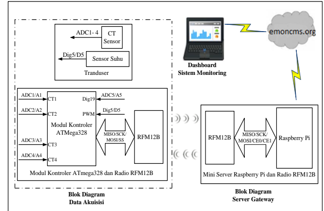
Gambar 1. Blok Diagram Sistem Monitor
